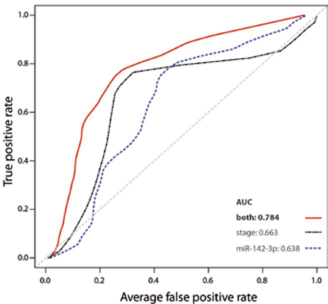
Figure 3: Improving prediction of recurrence in patients by using miRNA and stage (red line) in comparison to either miR-142-3p levels (blue line) or staging (black line) alone
