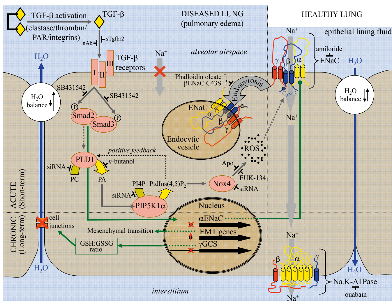
Figure 4. TGF- \beta directs ENaC trafficking: implications for disturbed alveolar ion and fluid transport in acute lung injury. In healthy lungs, latent TGF- \beta is inactive, and the Na + /K + -ATPase and ENaC drive Na + absorption, maintaining fluid influx and reabsorption in equilibrium, and epithelial lining fluid volume at an appropriate level. After activation of latent TGF- \beta by elastase-, integrin- or protease-activated receptor (PAR)-dependent mechanisms in acute lung injury an acute effect of TGF- \beta on alveolar fluid reabsorption was observed. In the unique signaling pathway delineated (dark gray arrows), TGF- \beta , acting through the type I TGF- \beta receptor, induces Smad2/3 phosphorylation, which activates PLD1, which generates PA from phosphatidylcholine (PC). PA activates PIP5K1 \alpha , which drives NOX4 activation, perhaps by PtdIns(4,5)P 2 formation from phosphatidylinositol 4'-monophosphate (PI4P). Activated NOX4 generates ROS, which promote \beta ENaC internalization that is dependent on Cys43, which leads to loss of Na + -absorbing capacity of the epithelial cell and alveolar flooding, promoting persistence of alveolar edema. (Peters DM, Vadasz I, Wujak L, Wygrecka M, Olschewski A, Becker C, Herold S, Papp R, Mayer K, Rummel S, Brandes RP, Günther A, Waldegger S, Eickelberg O, Seeger W, Morty RE. TGF- \beta directs ENaC trafficking: implications for disturbed alveolar ion and fluid transport in acute lung injury. Proc Natl Acad Sci U S A 2014; 111(3):E374-83)
