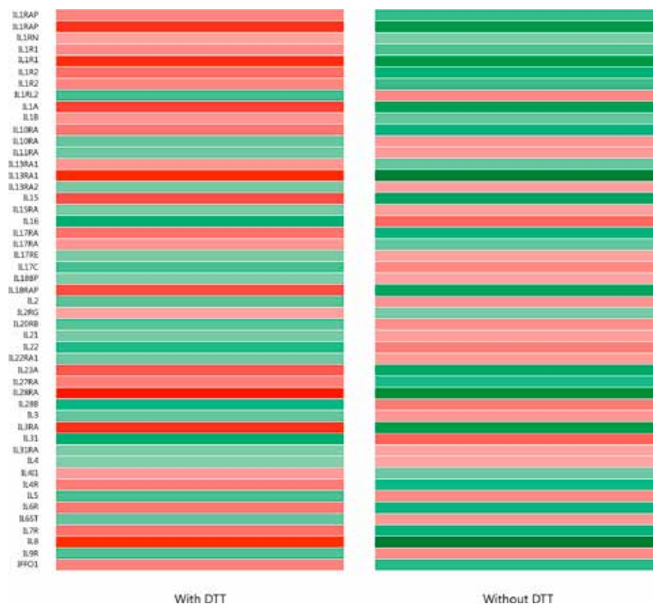
Figure 5. Heat map of transcriptome analysis of HOPE-preserved induced-sputum RNA processed with and without DTT. Agilent ( 4 \times 44K ) human whole genome arrays were used. Analysis of the results was performed with a fold-change analysis using Gene-Spring 12 software. Red color intensity indicates higher expression, green color intensity indicates lower expression and white indicates a medium level of expression of a gene in the comparison of both groups. Gene description is shown on the left-hand side.
