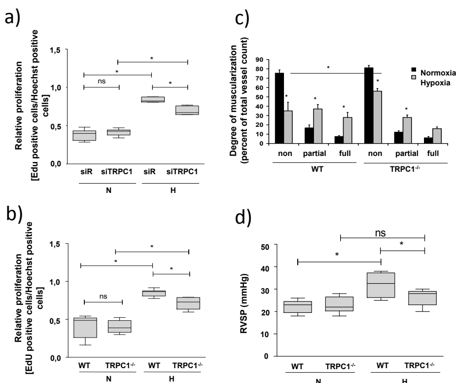
Figure 3. a) and b) Hypoxia (H, 24h, 1% O 2 ) -induced proliferation of (a) murine PASMC after knockdown of TRPC1 expression (siTRPC1) compared to control (siR) (n=4-5) and (b) murine PASMC isolated from WT and TRPC1 -/- (n=5-7) assessed by cell counting using 5-ethynyl-uridine (EdU) based proliferation assay. c) Degree of muscularization in small pulmonary vessels (external diameter of 20-70µm) from WT and TRPC1 -/- mice exposed to normoxia (21d; 21% O 2 ) or chronic hypoxia (21d; 10% O 2 ). The proportion of fully muscularized (full), partially muscularized (partial) and non muscularized (non) vessels is given in percentage of total vessel count (n=5). d) Right ventricular systolic pressure (RVSP) in WT and TRPC1 -/- mice kept under normoxic (N, 21d; 21% O 2 ) or chronic hypoxic (H, 21d; 10% O 2 ) conditions (n=7). Adapted with permission of the American Thoracic Society. Copyright © 2013 American Thoracic Society. Malczyk, et al., 2013. Classical transient receptor potential channel 1 in hypoxia-induced pulmonary hypertension. 188: 1451-59. Official Journal of the American Thoracic Society.
